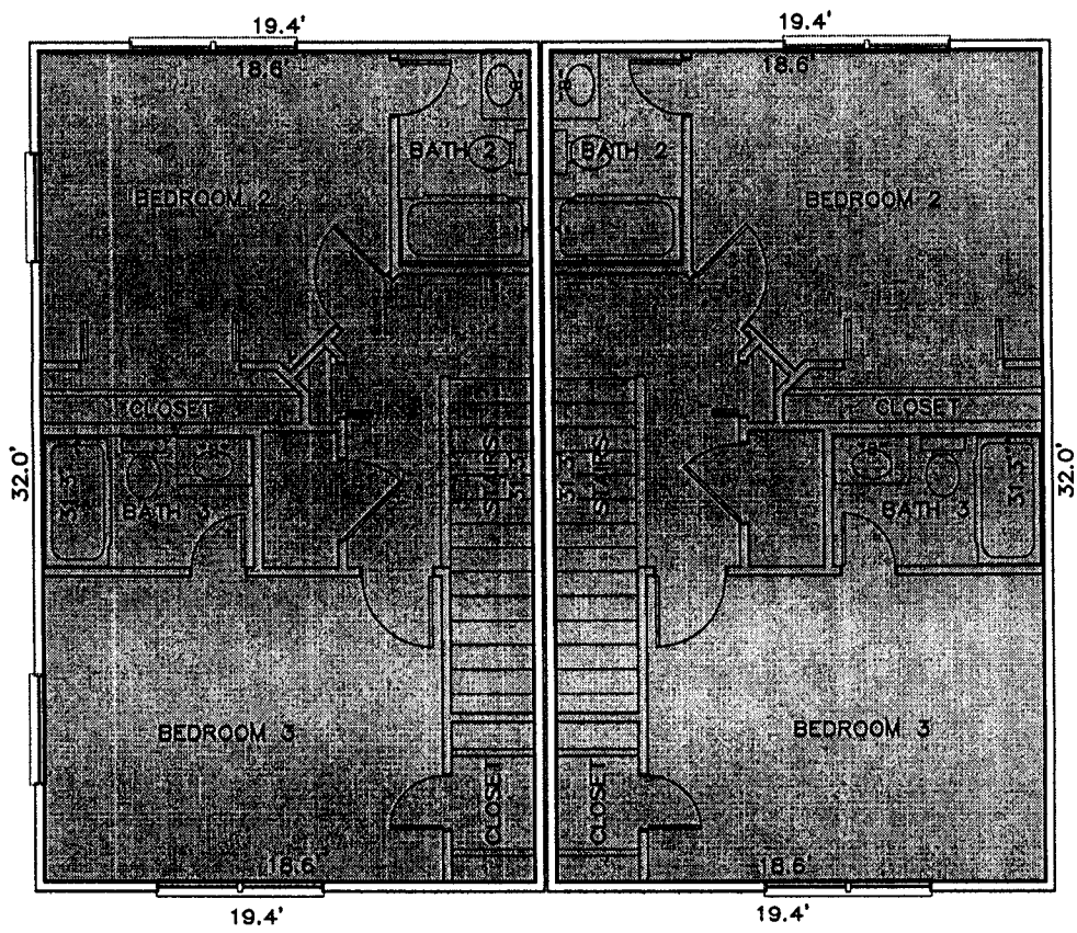
SECOND FLOOR PLAN (TYPICAL)
