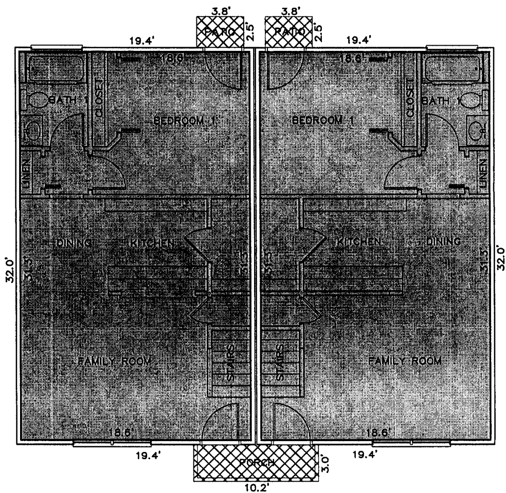
FIRST FLOOR PLAN (TYPICAL)
